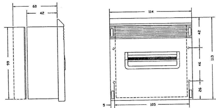
ALL DIMENSIONS IN MILLIMETERS
